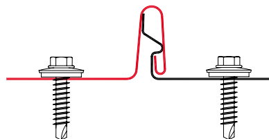
FIGURE 2. LOCK IN STANDING SEAM ROOF PANEL ELEGANT WITH VISIBLE ATTACHMENT
