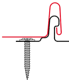
FIGURE 1. LOCK IN STANDING SEAM ROOF PANEL ELEGANT WITH HIDDEN ATTACHMENT
